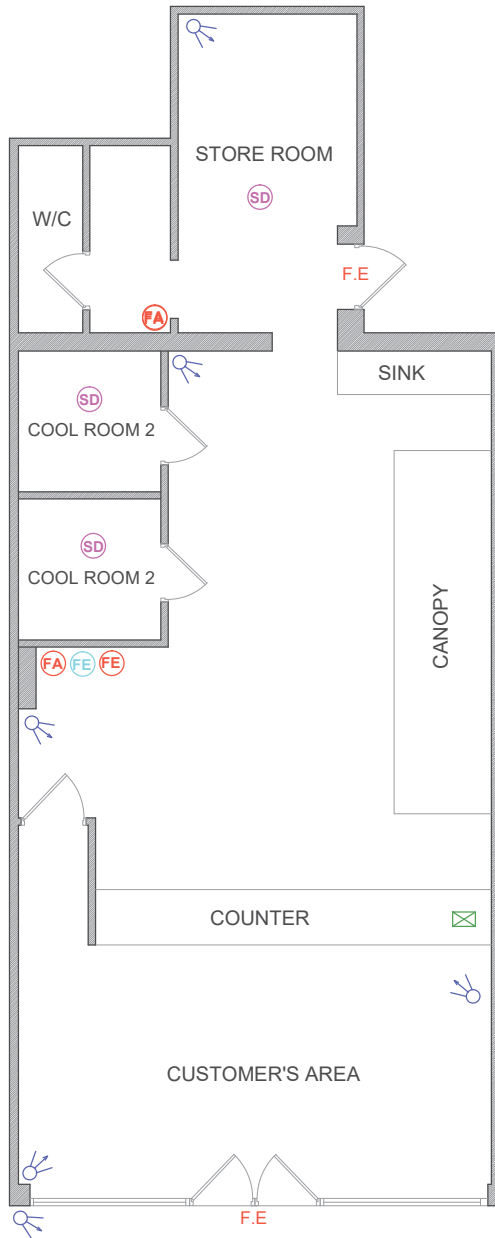
SHOP FLOOR PLAN Scale 1:100
